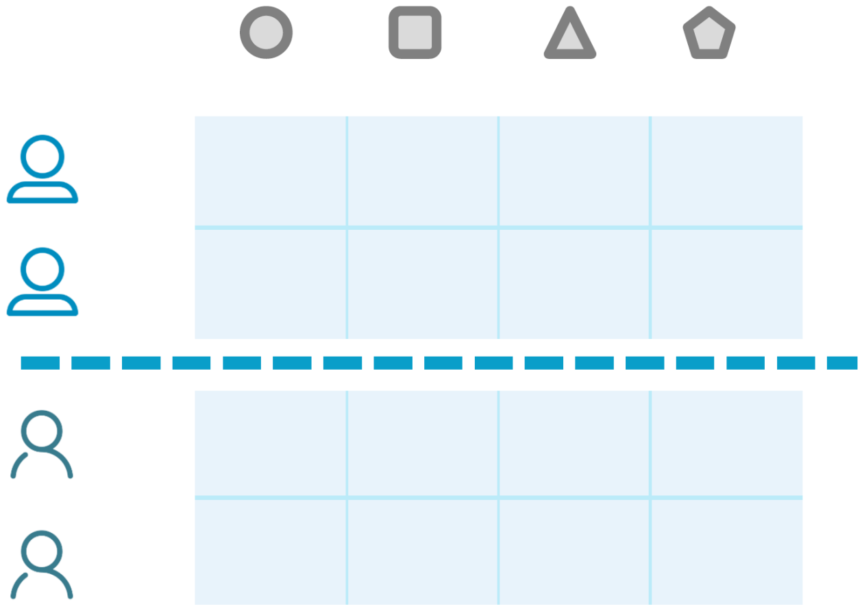
Fig. 4.9: Horizontally-partitioned data
