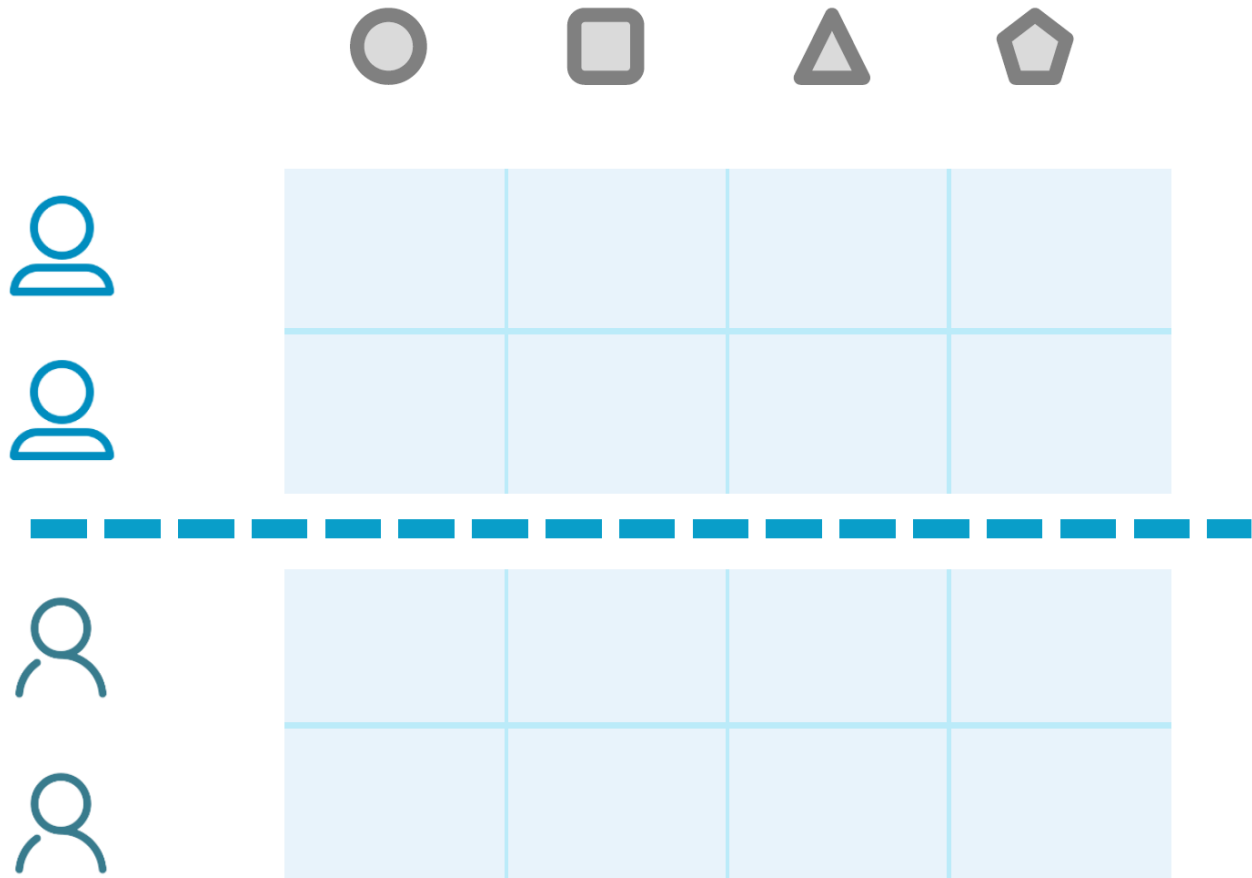
Fig. 4.11: Horizontally-partitioned data
