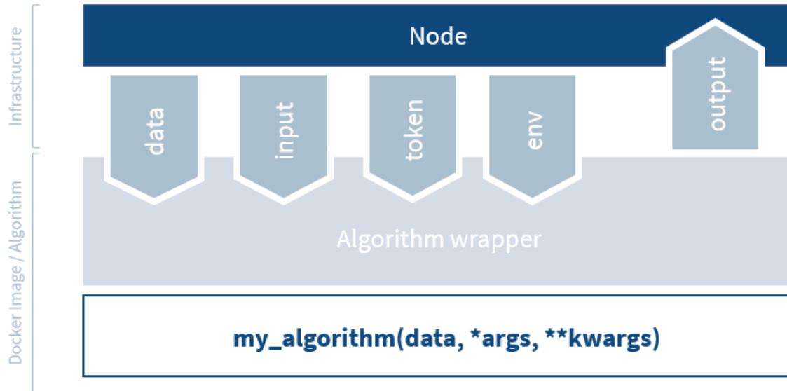
Fig. 4.7: The algorithm wrapper handles algorithm input and output.
